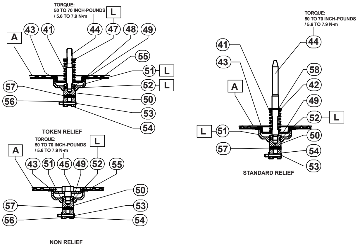
Figure 8. CS400 Series Regulator Assemblies (continued)
