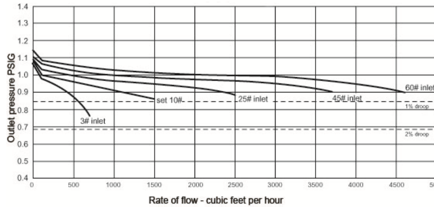
Relief Curves
