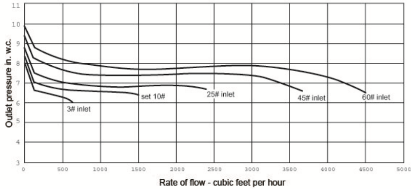
Relief Curves
