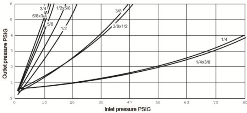
Relief Curves
