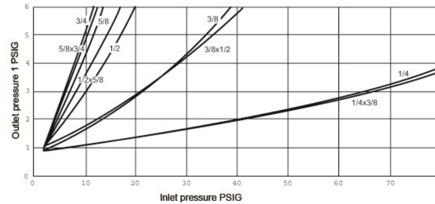
Relief Curves
