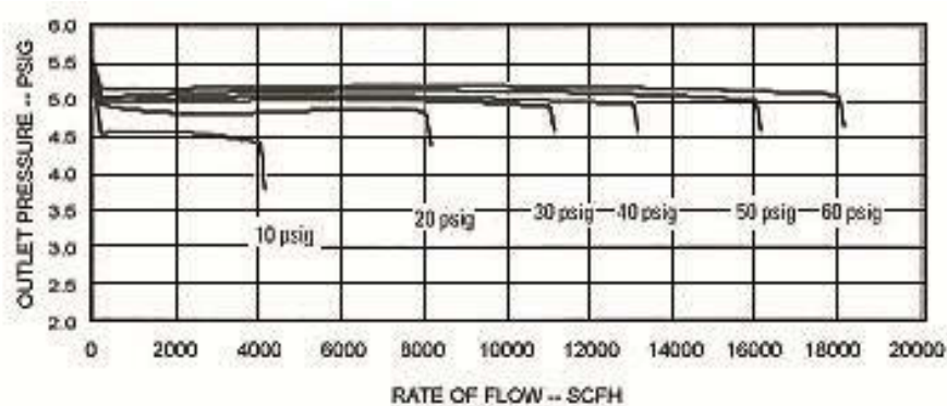
Performance Curves
