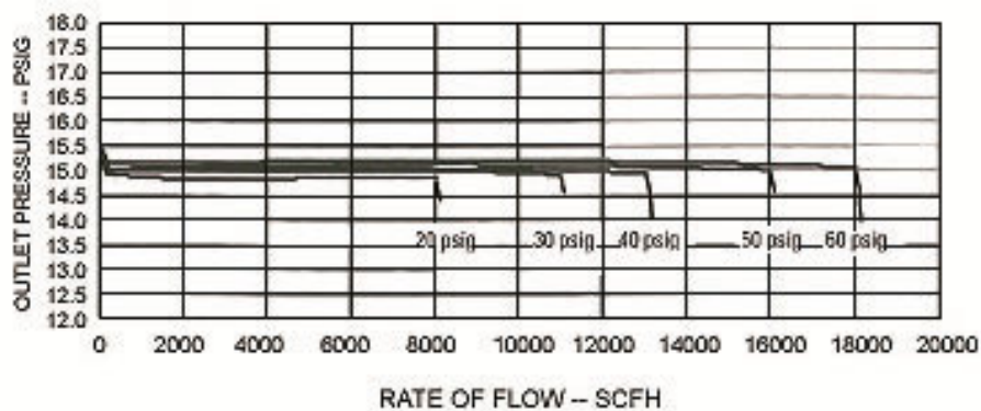
Performance Curves
